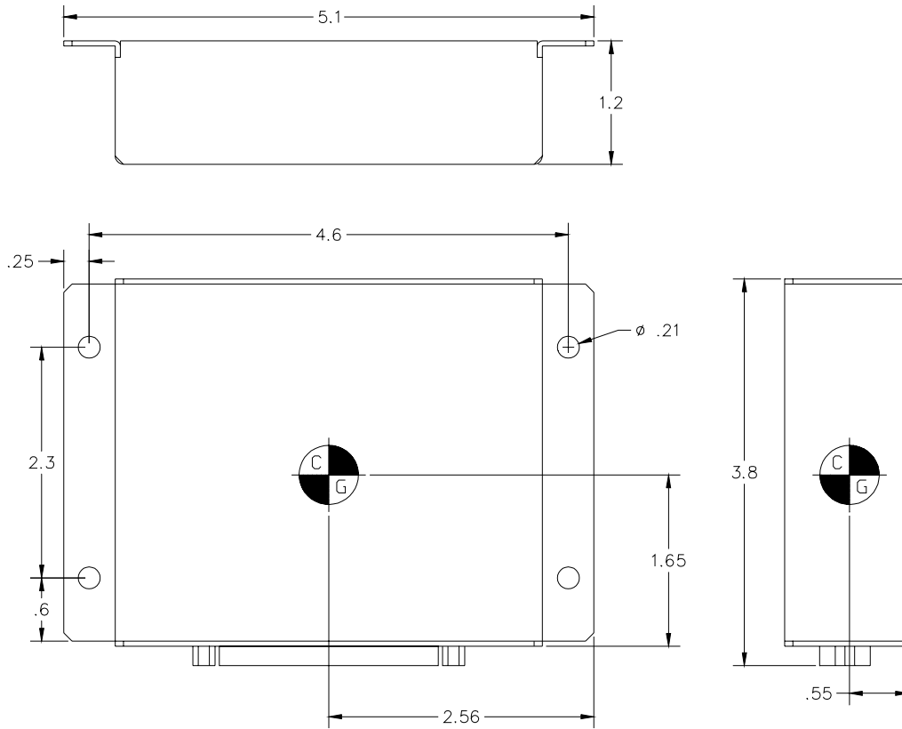
SAS 1-24 Mechanical Dimensions
